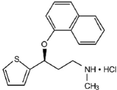
duloxetine
